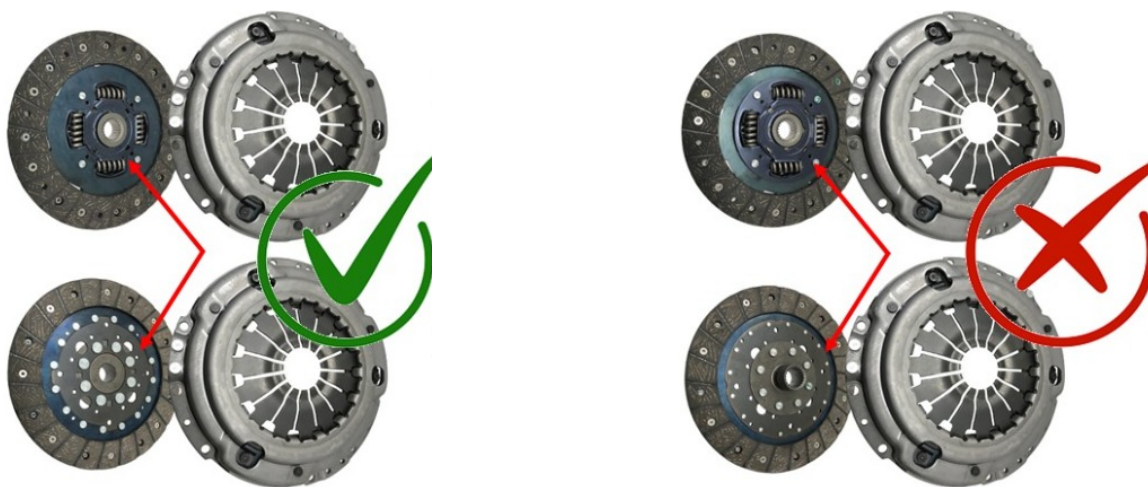
Left: correct installation. Right: incorrect. Top: NAK06-882S; bottom: NAK06-877S.
